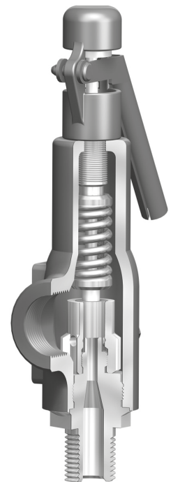
Fig. 969 open lifting device
