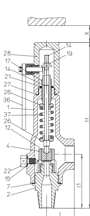
Fig. ... 966 closed lifting device
